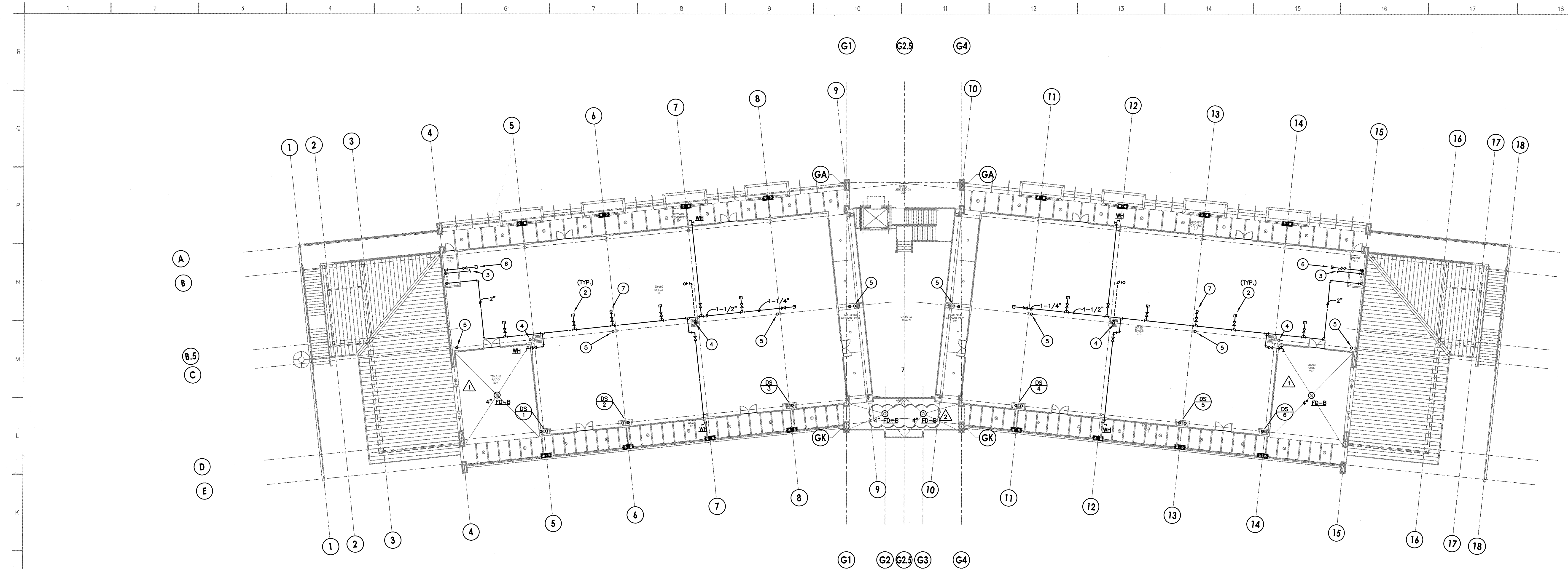
01 SECOND FLOOR PLUMBING PLAN Scale: 1/16"=1'-0"
