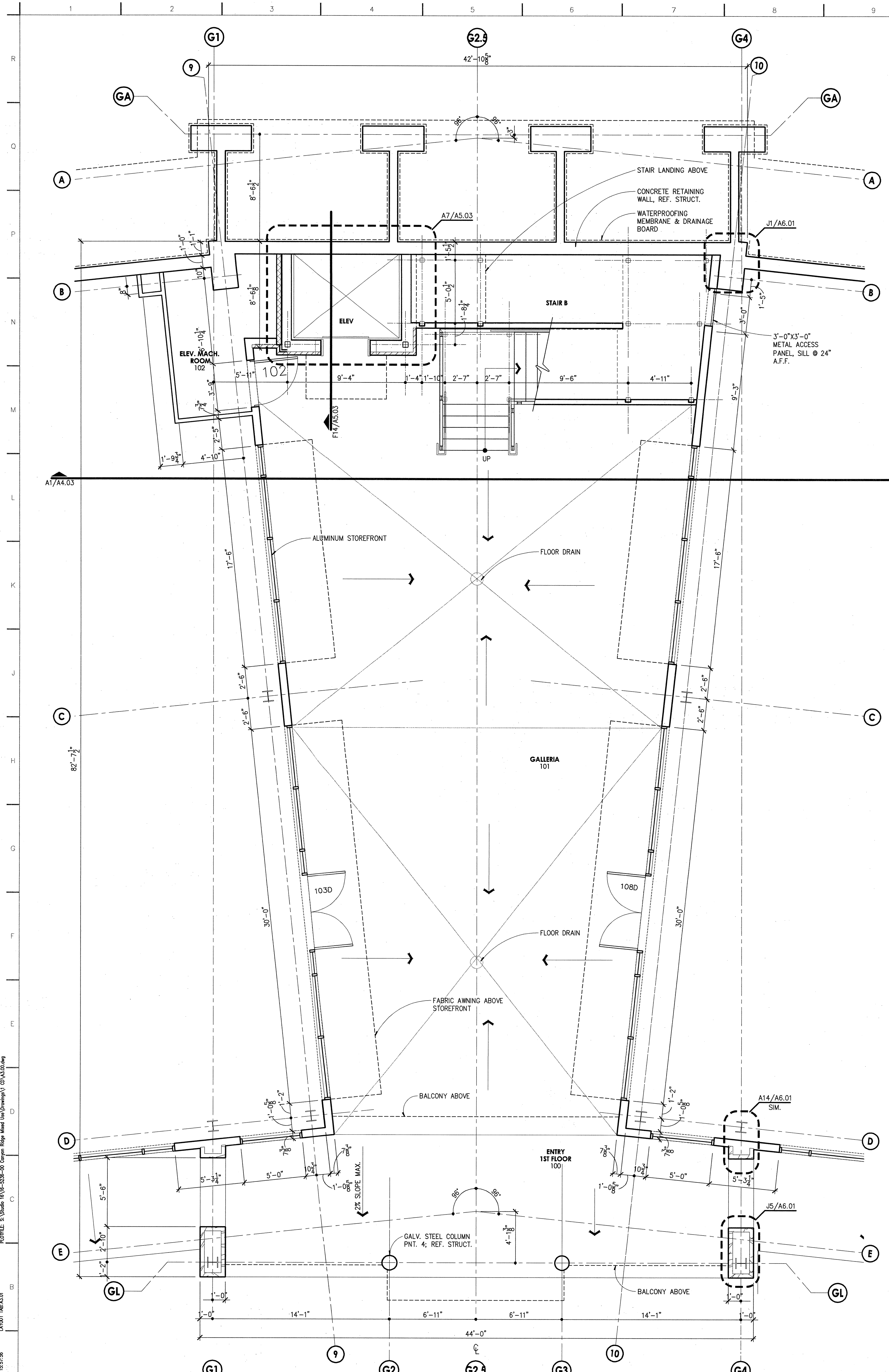
A1 ENLARGED PLAN - GALLERIA 1ST FLOOR 1/4"=1'-0"
