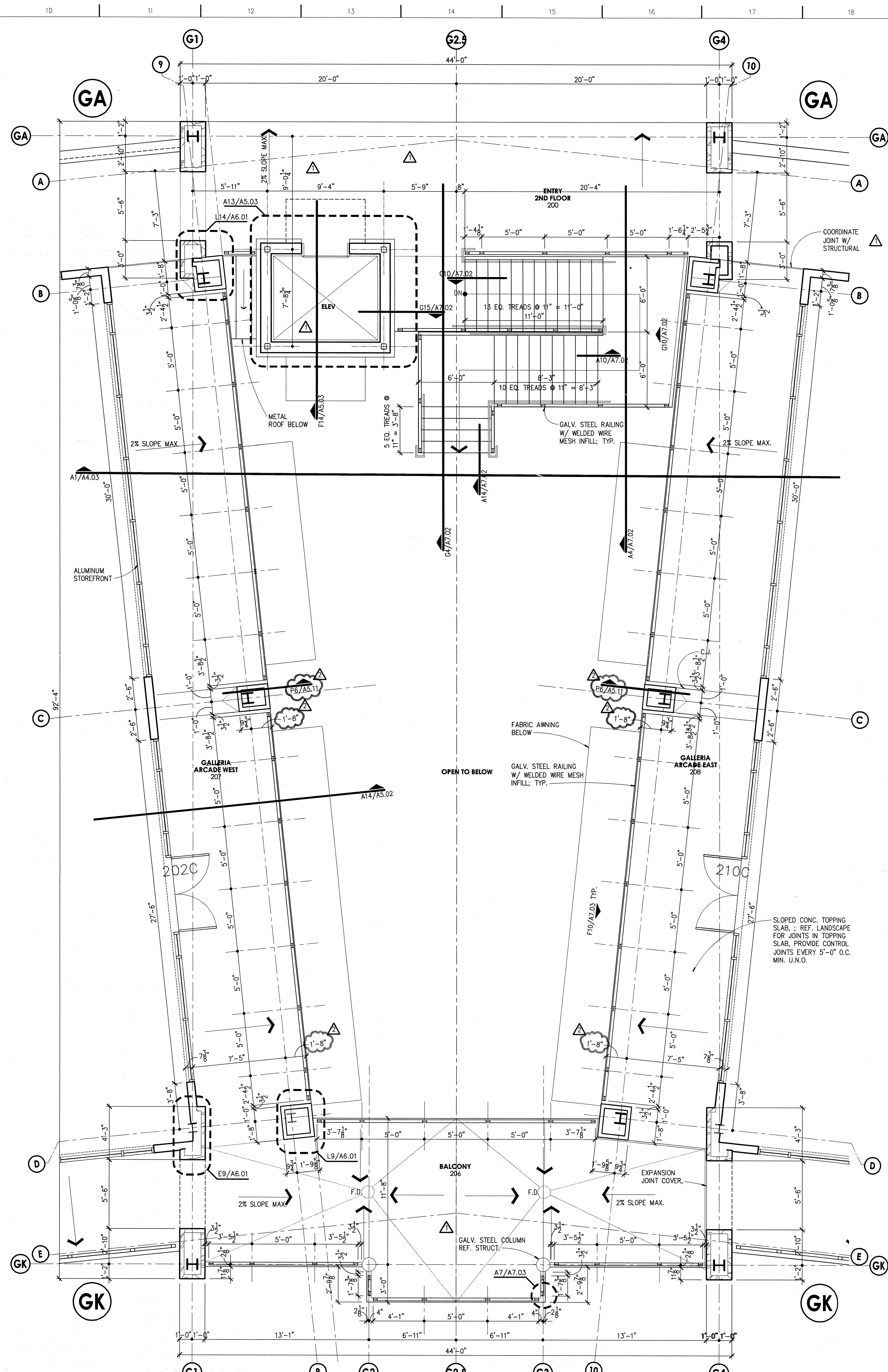
A10 ENLARGED PLAN - GALLERIA 2ND FLOOR 1/4"=1'-0"
