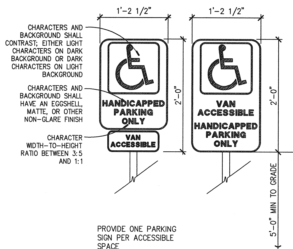
PARKING SIGNAGE Scale: 1"=1'-0"
