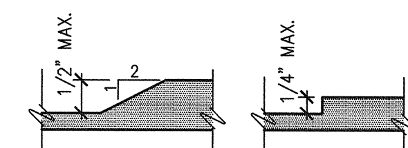
LEVEL CHANGES Scale: FULL SCALE
