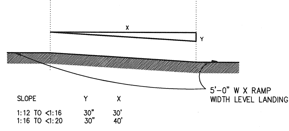
RAMP SLOPES & LANDINGS Scale: NONE
