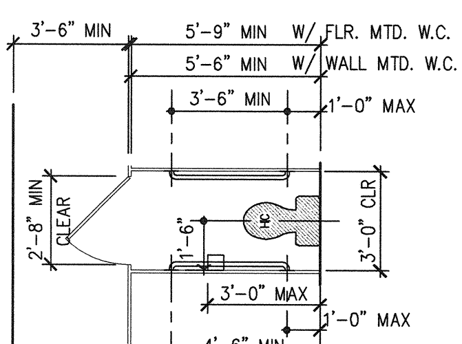
ALTERNATE TOILET STALL Scale: 1/4"=1'-0"
