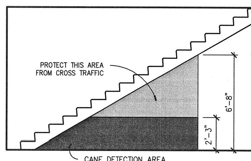
OVERHEAD HAZARDS Scale: 1/4"=1'-0"
