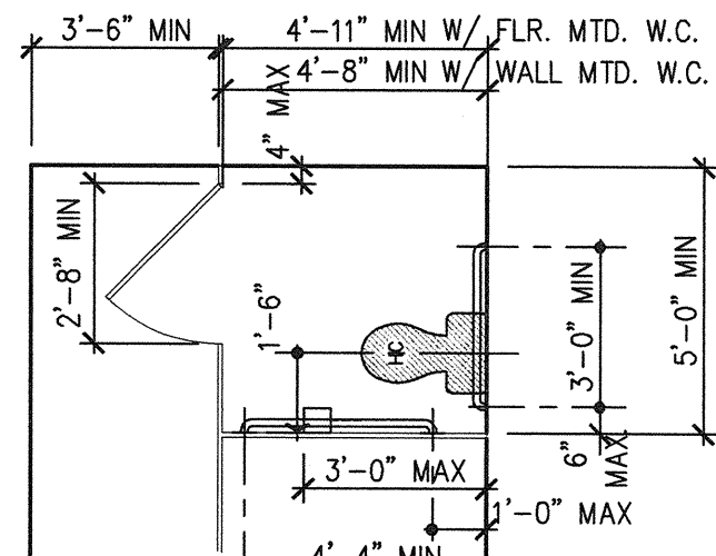
STANDARD TOILET STALL Scale: 1/4"=1'-0"
