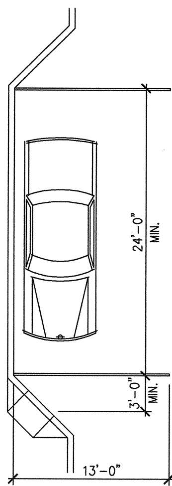
PARKING SPACE DIMENSIONS Scale: 1/8"=1'-0"
