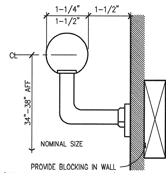
HANDRAIL @ RAMP OR STAIR Scale: HALF SCALE
