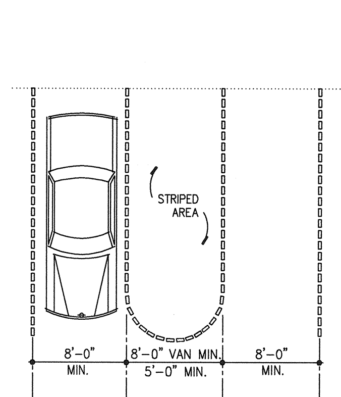
PARKING SPACE DIMENSIONS Scale: 1/8"=1'-0"
