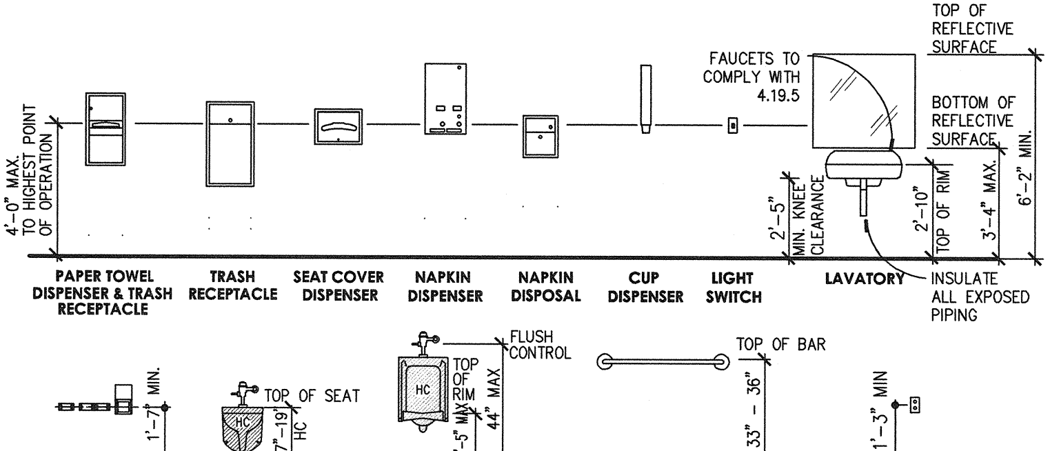
STANDARD MOUNTING HEIGHTS Scale: 1/4"=1'-0"
