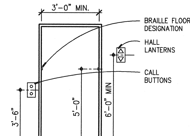
ELEVATOR ENTRANCES Scale: 1/4"=1'-0"
