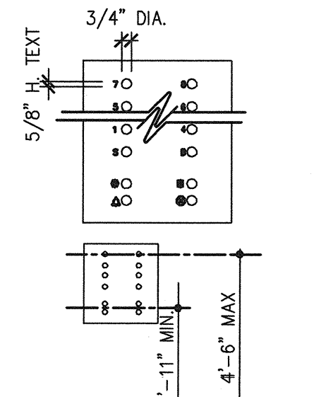
ELEVATOR CONTROL HEIGHT Scale: 1/4"=1'-0"
