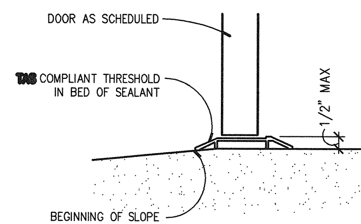
THRESHOLD Scale: FULL SCALE
