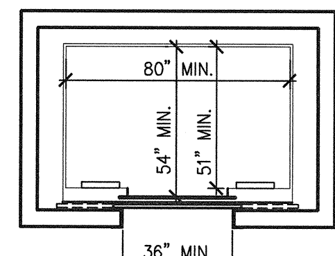
ELEVATOR CAB CLEARANCES Scale: 1/4"=1'-0"
