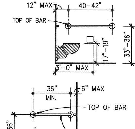
TOILET STALL ELEVATIONS Scale: 1/4"=1'-0"
