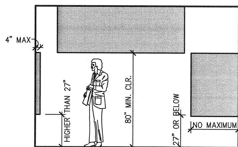
PROTRUDING HAZARDS Scale: 1/4"=1'-0"
