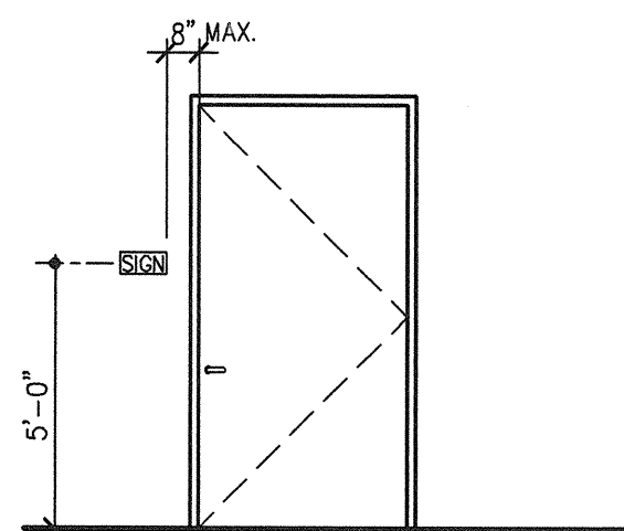
SIGNAGE MOUNTING HEIGHT Scale: 1/4"=1'-0"
